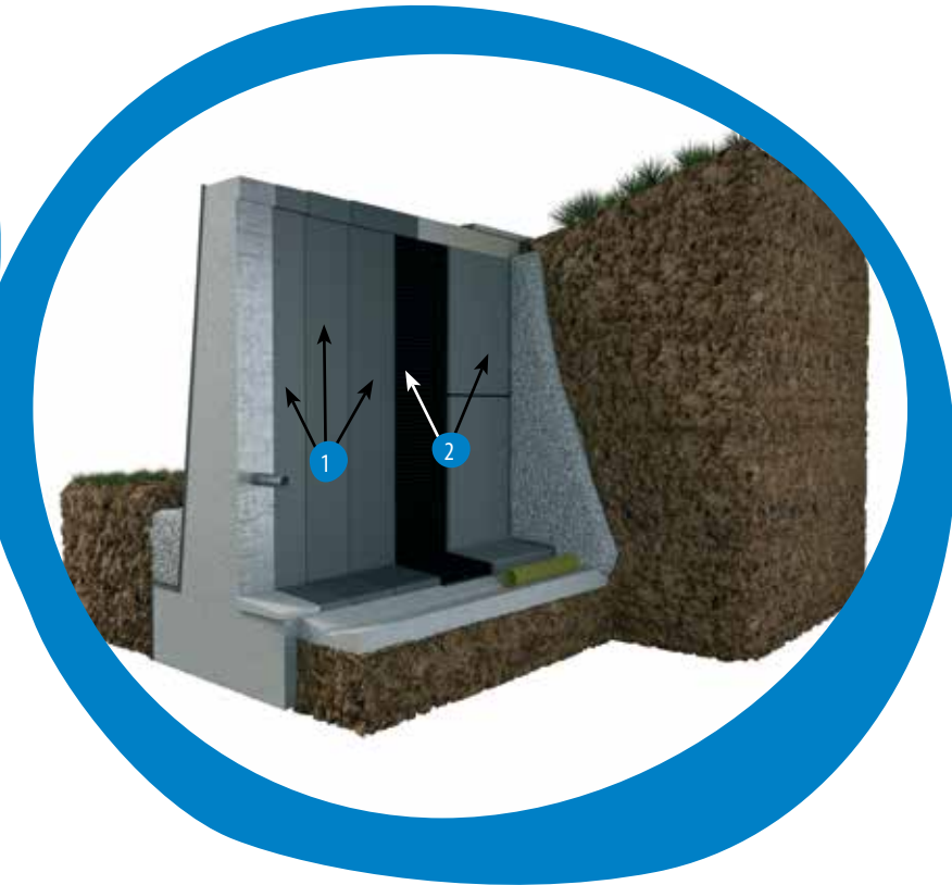
1. Waterproofing: 3x application of HYDROSOL Classic 2. Waterproofing protection
